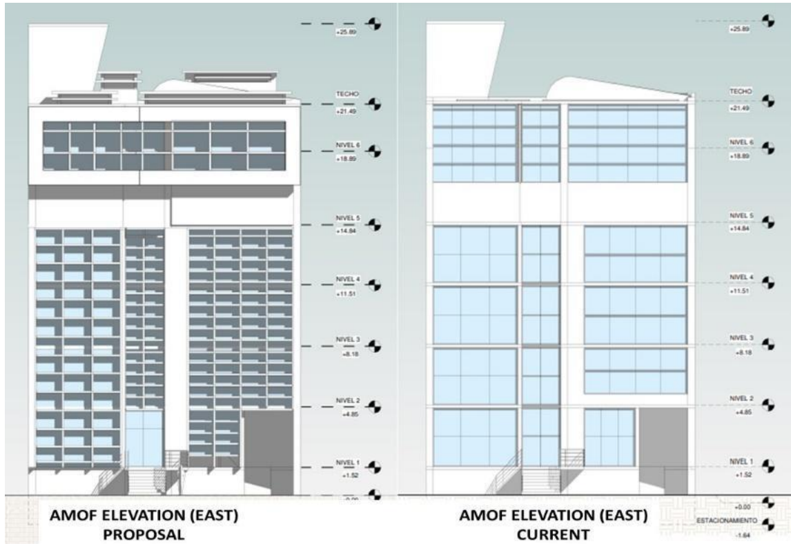
Figure 10. AMOF Building - Proposal and Current (Facades), Miraflores. Based on Autodesk Revit 2020 software. Own preparation.
